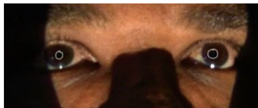
Figure 4: Pupil size in dim illumination.
